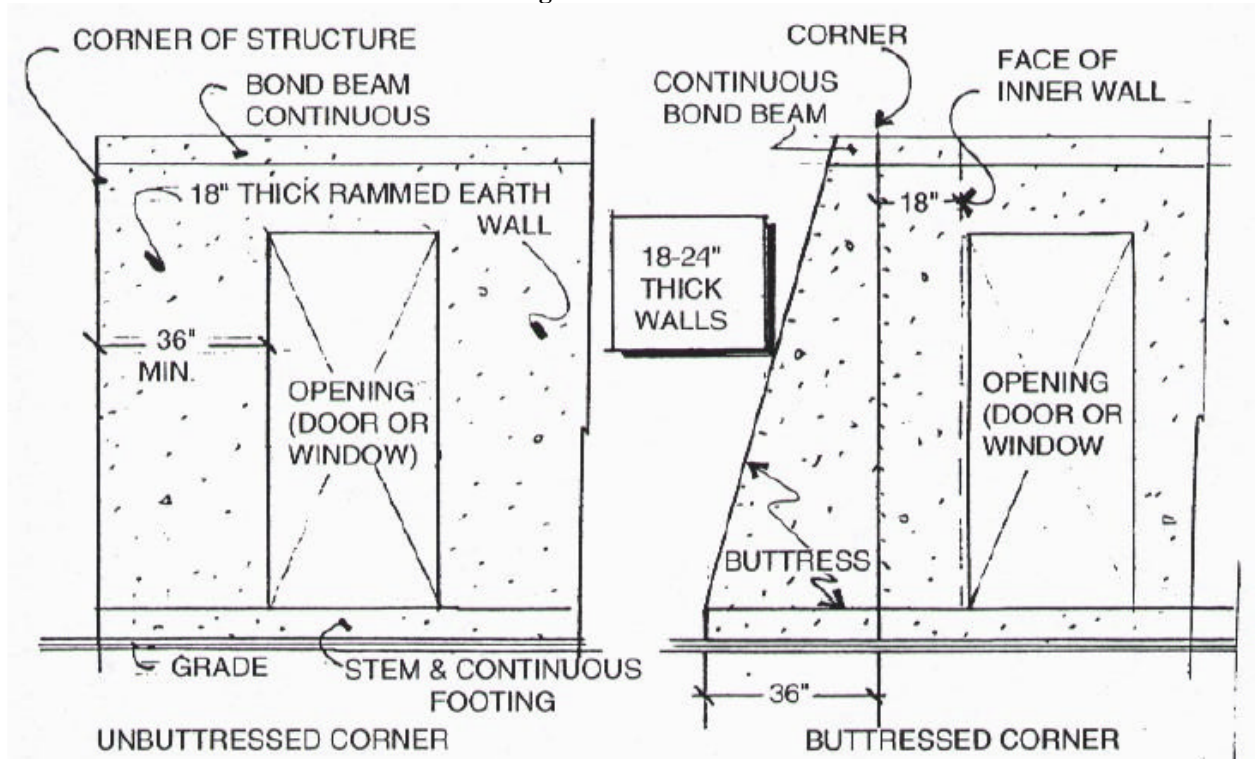
Figure 1 – Buttress:
