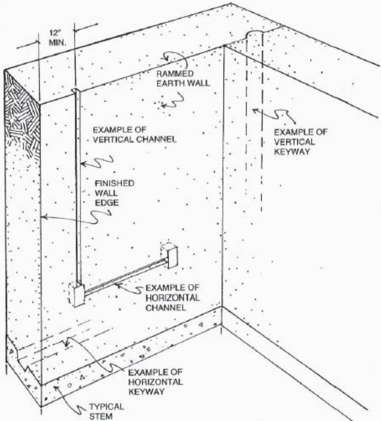
14.7.4.32 FIGURE 3 - KEYWAY
